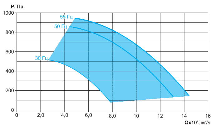
VCR-830/56-ПЦ-3,0/1500/220-380
