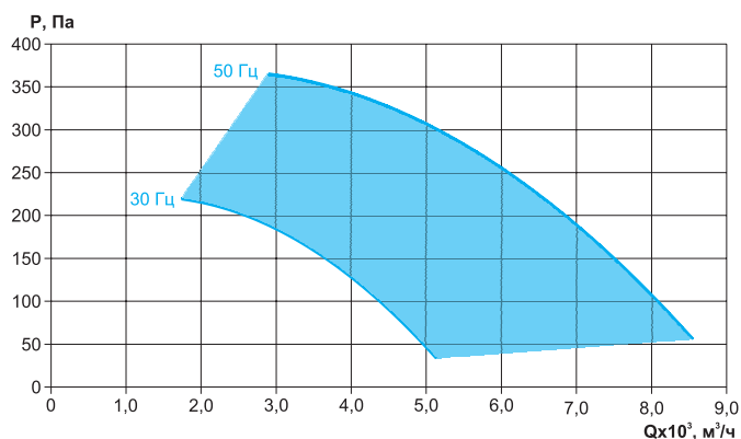
VCR-830/56-ПЦ-1,5/1000/220-380
